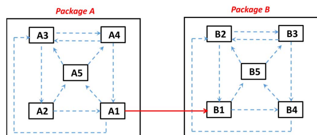
Fig. 1. Aggregation of metrics to the architecture level
